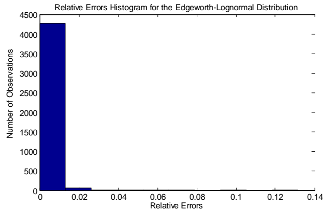
Figure 2: Histogram of relative errors of the Edgeworth approximation
